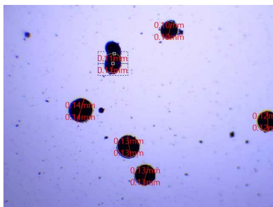
Representation of particle size of IZ (measured by light microscope equipped with appropriate camera and software)
